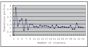
Fig. 5. Transition profile diagram of dataset III
