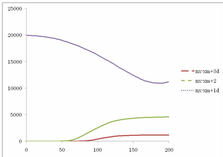
Fig. 2. Learning history and number of excludable outliers. Abbreviations: nx-xm+\alpha.d (number of outliers with) \epsilon_i > \epsilon_{av} + \alpha \cdot \sigma(\epsilon) .
