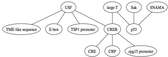
Fig. 2. Preliminary Protein Binding Network of CREB
