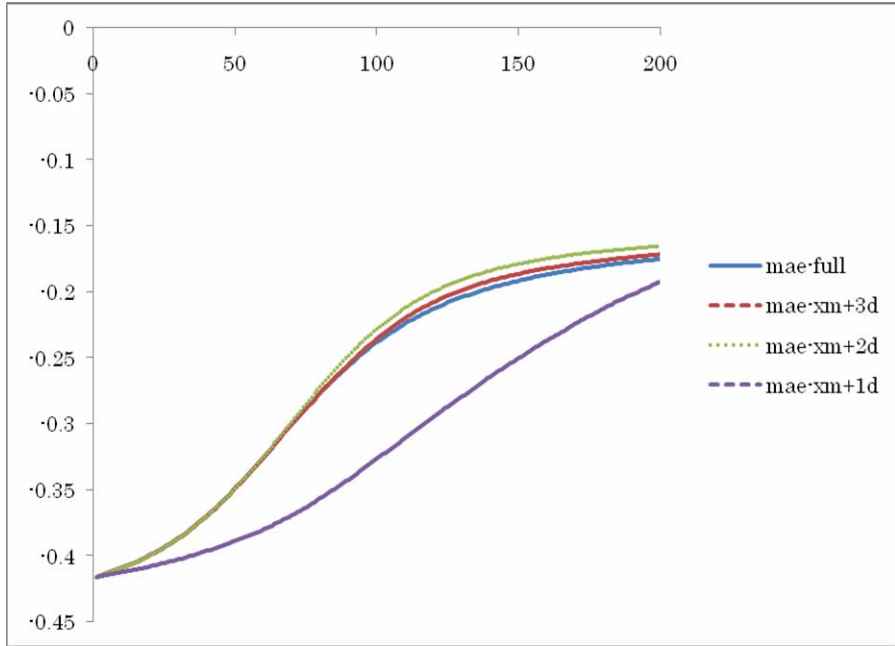
Fig. 1. Learning history of mean absolute error in the test data (generalization). Abbreviation (mae-full; Mean Absolute Error in test data without error exclusion, mae-xm+ \alpha .d; MAE in test data when training points with \epsilon_i > \epsilon_{av} + \alpha \cdot \sigma(\epsilon) were excluded). MAE values are marked as negative to contrast them from correlation and other accuracy scores to indicate that a smaller MAE means better prediction.
