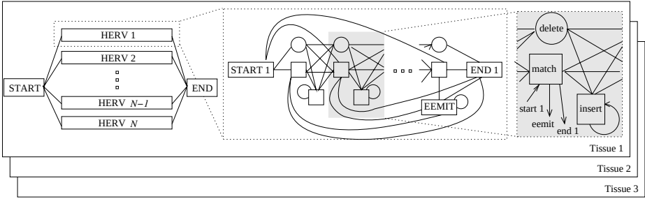
Fig. 1. The structure of the HMM mixture. The model is constrained by sharing parameters. The shaded box is the basic block of the sub-HMM and is repeated length-2 times. It is identical in all sub-HMMs; all other parameters are shared except the emission distribution of the match state which varies between blocks, according to the HERV sequence each sub-HMM corresponds to. EEMIT-state emits the low-quality end part. The plates illustrate that the same model is learned separately for each tissue.
