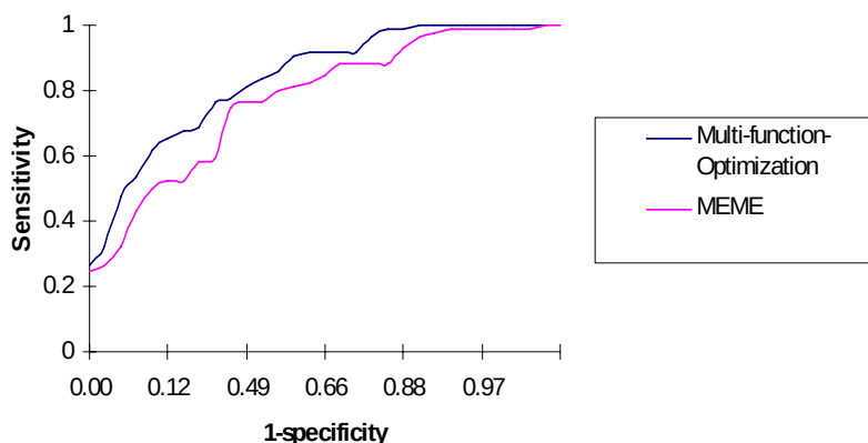
Fig. 2. The ROC plot illustrating the specificity and sensitivity values at different thresholds
